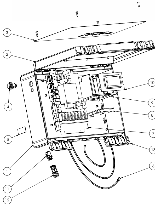
DIAGRAM 1 - DCCU
