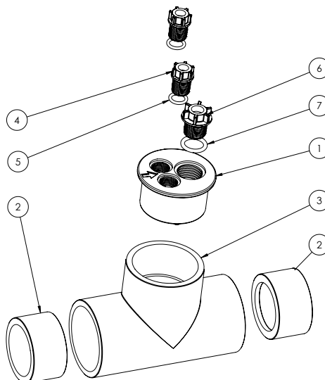
DIAGRAM 2 - Flow Cell
